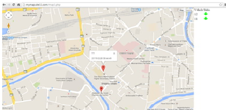
Fig6. Web application
