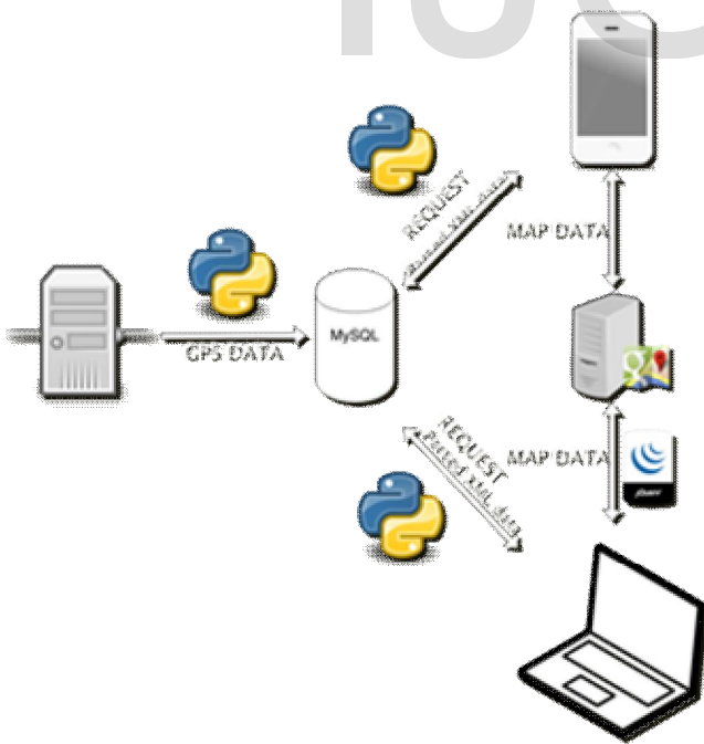
Fig4. Client-Server Architecture
