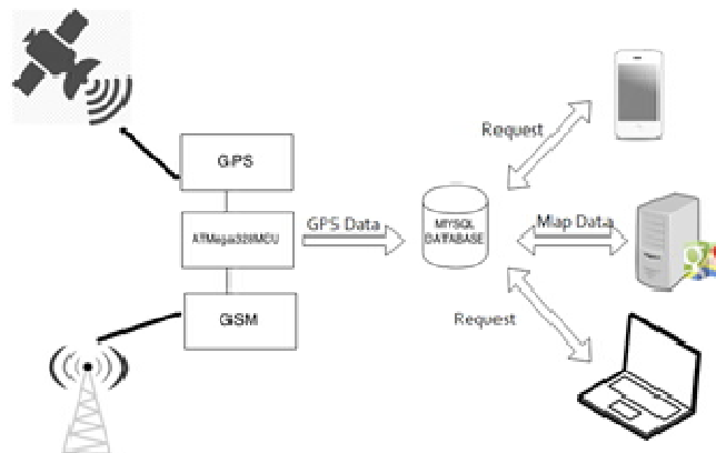
Fig1. Architecture of vehicle tracking system The hardware used here are GPS Module, GSM Module and ATMega328 Microcontroller.
